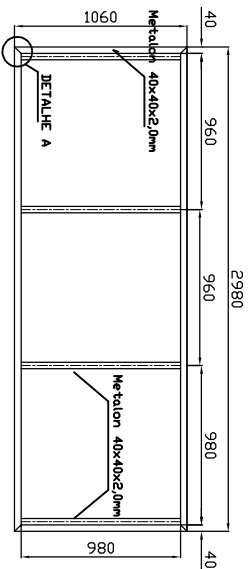
VISTA FRONTAL
